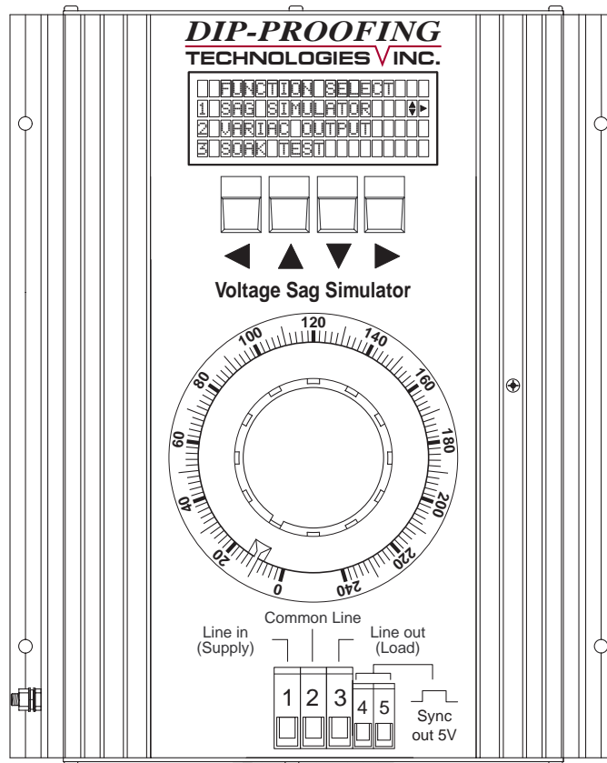
Fig 7 Controls & indicators
