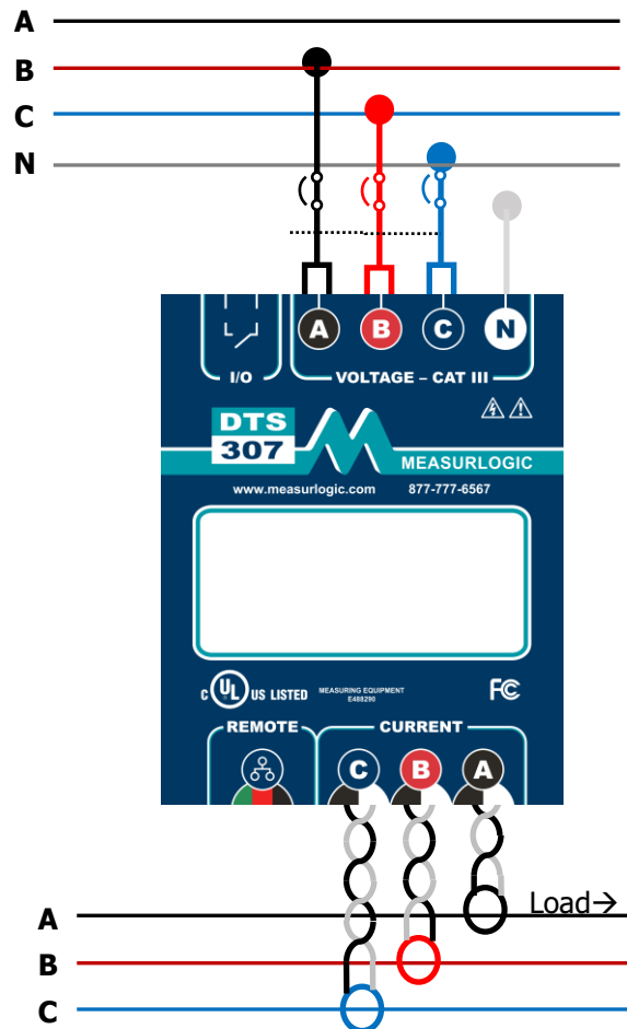
DTS 307 3-Phase 4 Wire (with Neutral)
