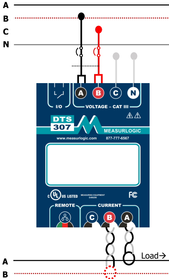
DTS 307 Single Phase 2/3 Wire Unused Voltage Inputs MUST be Connected to the Neutral Terminal
