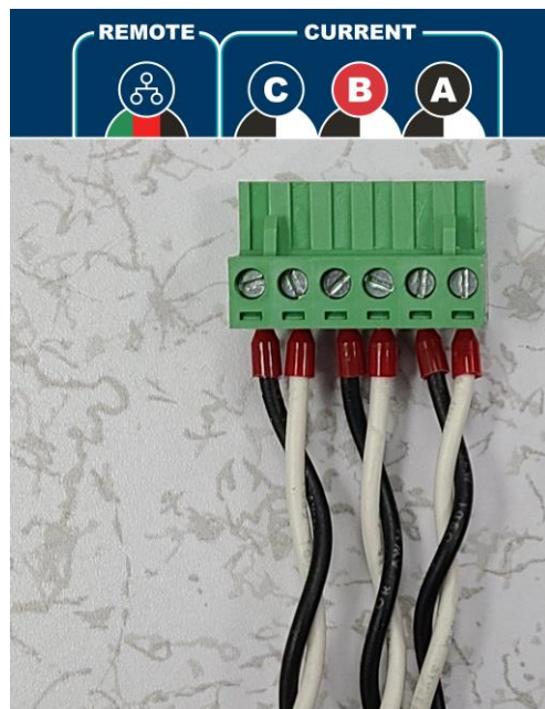
Split and Solid Core CTs
