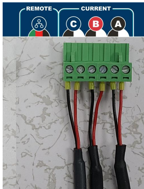
Rogowski Coil CTs
